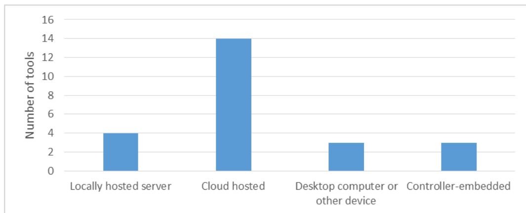
Figure 3. Software location
